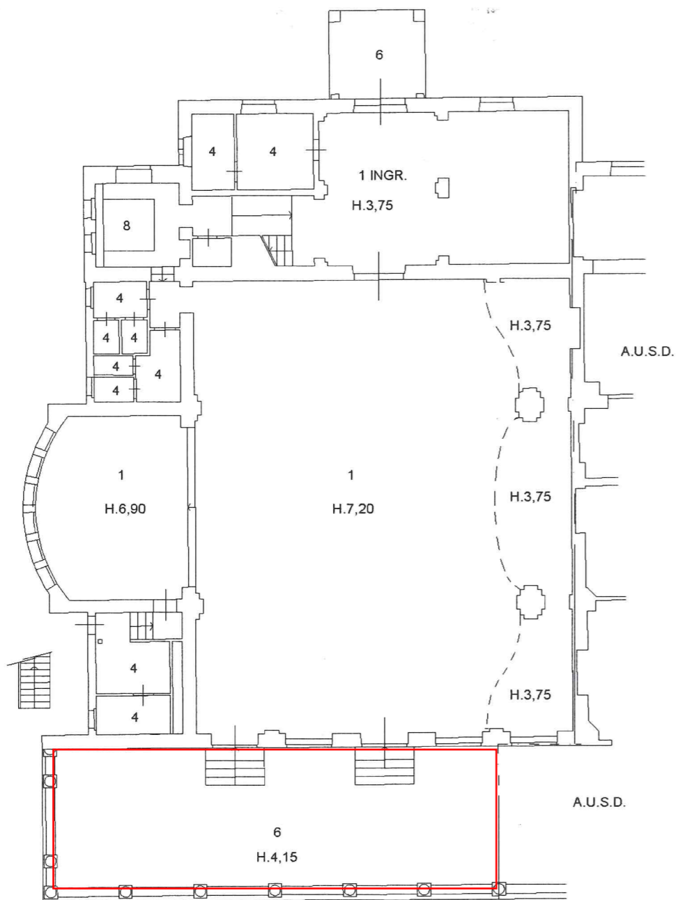
PIANO TERRA
